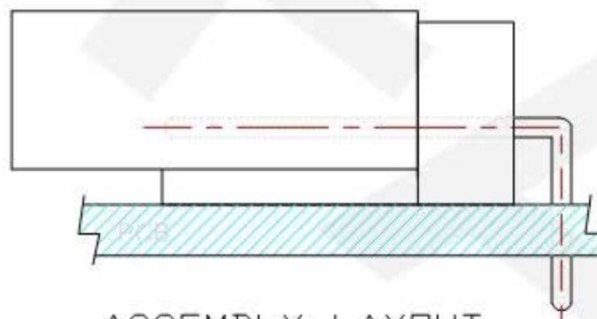
ASSEMBLY LAYOUT
